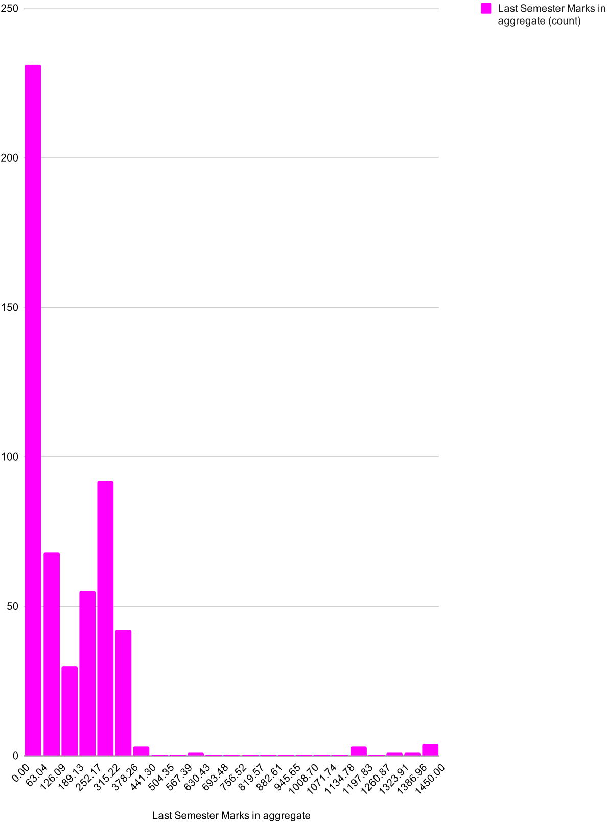
Histogram of Last Semester Marks in aggregate
